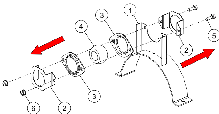
DISASSEMBLED BEARING
